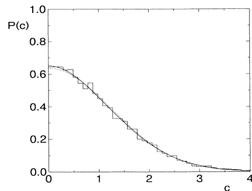
FIG. 1. The normalized histogram of avoided crossings for the kicked-top model Eq. (3.1). Solid and dotted lines compare two theoretical probability-density distributions resulting from Eqs. (2.15) and (2.6), respectively. The horizontal axis is in dimensionless crossings c = C/\bar{C}^{KT} . Both theoretical distributions are expressed in respect to numerically found mean crossing. The data correspond to j = 50 odd-parity tops with k = 10, 11, \dots, 20 and the parameter \lambda = p \in [1.9, 2.6] interval.
